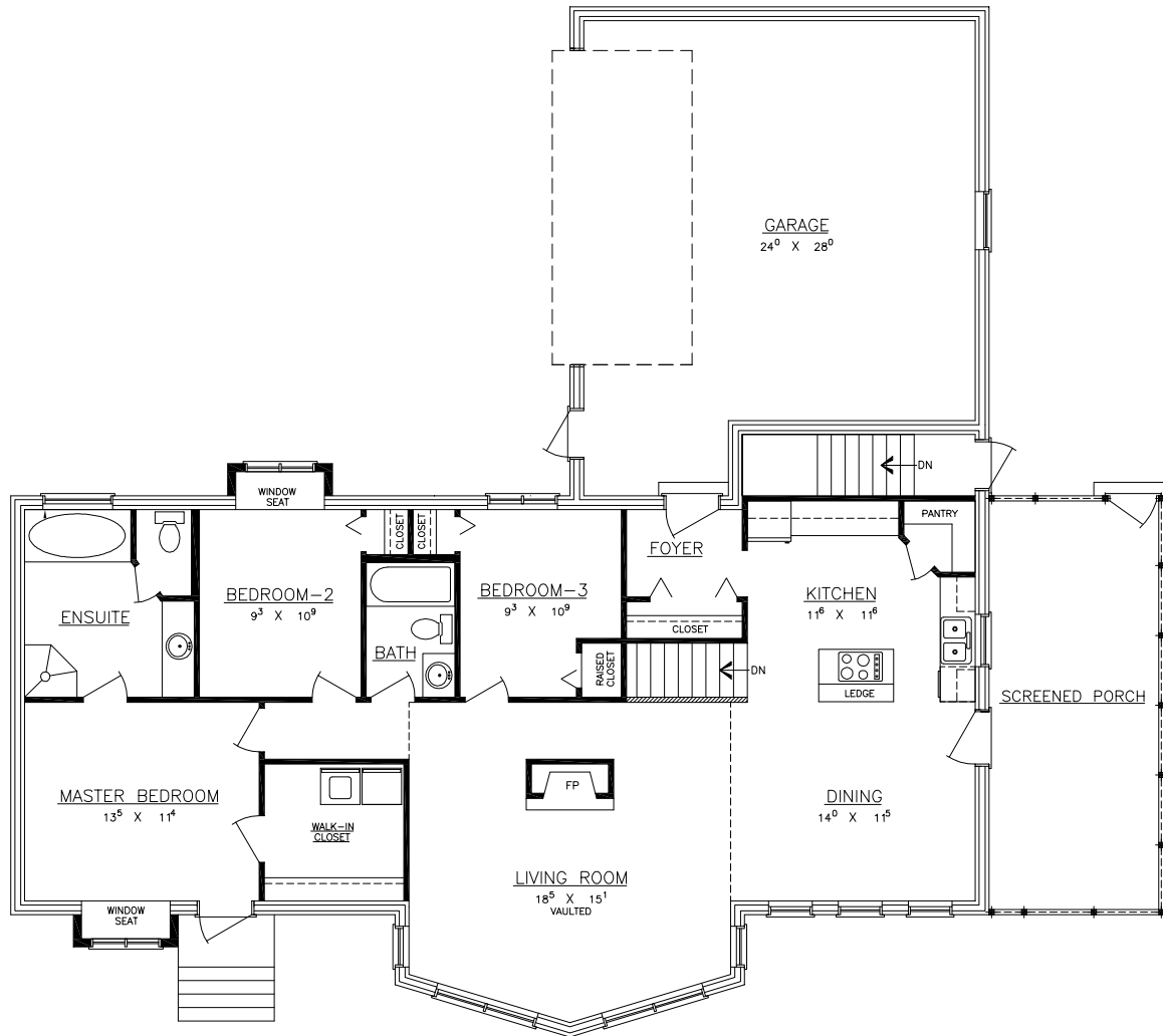
FLOOR PLAN
